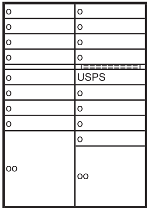
30 9/16" Model 4216-AB
