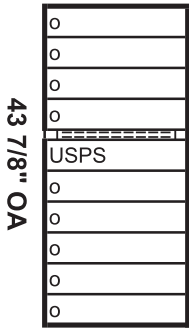
16 11/16" Model 4109-X
