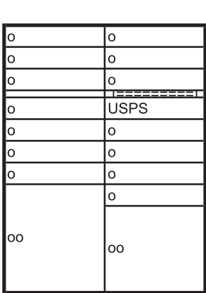
30 9/16" Model 4214-AB
